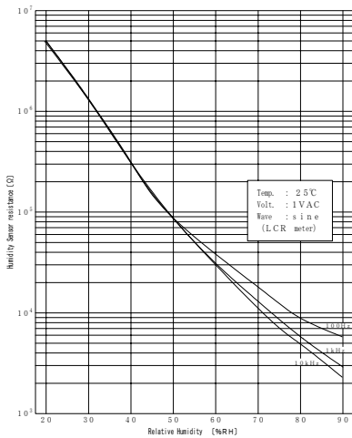
<Frequency Characteristics>
