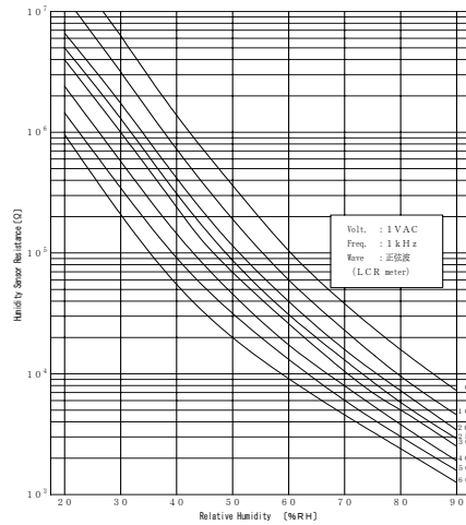
<Temperature Characteristics>
